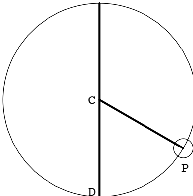
FIGURE 1. The pivot C of the pendulum moves vertically and periodically with period \frac{2\pi}{\mu} .
