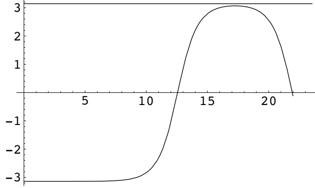
FIGURE 3. The solution with r = 0.001 that reaches the downward vertical position when t = 4\pi does not cross over the unstable equilibrium before t = 5\pi
