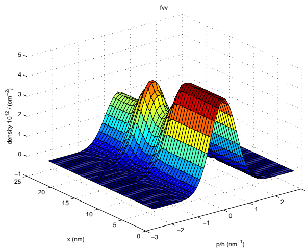
Figure 5: Thermal equilibrium Wigner function f_{2,2}
