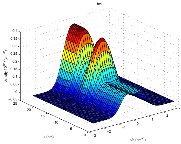
Figure 4: Thermal equilibrium Wigner function f_{1,1}
