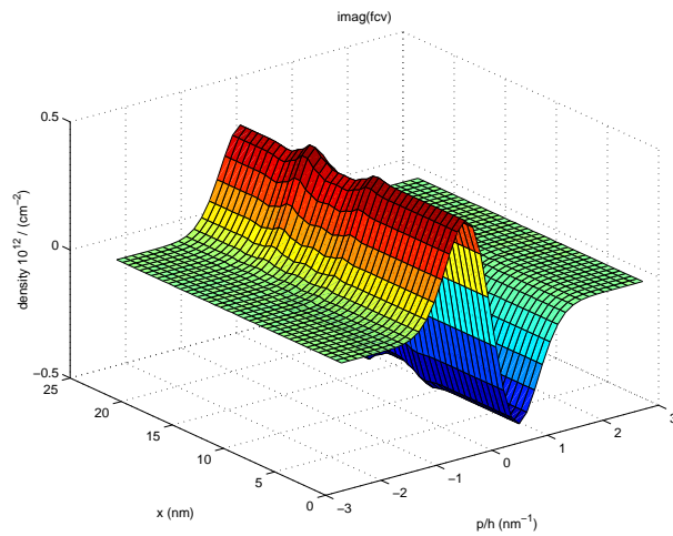
Figure 7: Imaginary part of thermal equilibrium Wigner function f_{1,2}
