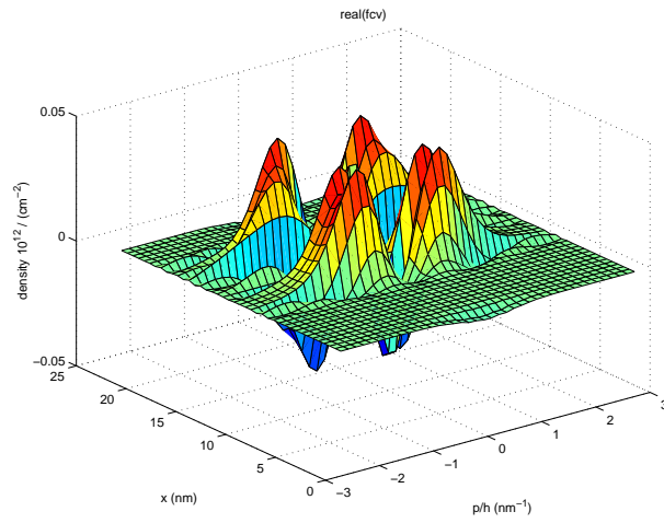
Figure 6: Real part of thermal equilibrium Wigner function f_{1,2}
