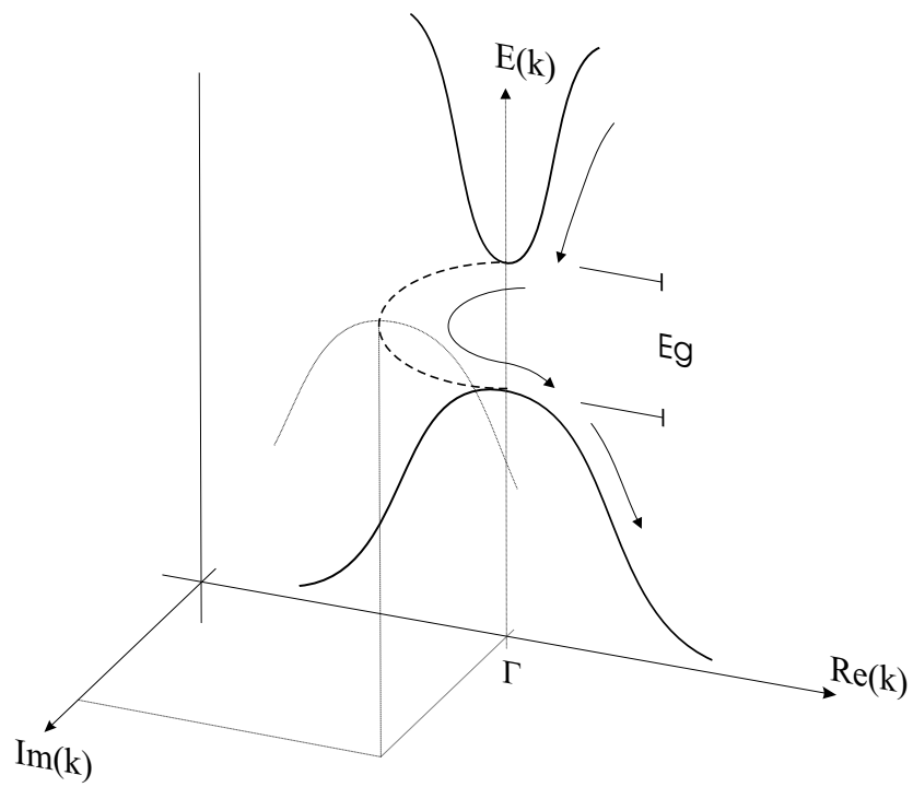
Figure 2: Dispersion diagram for real and imaginary values of k
