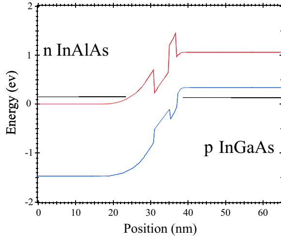
Figure 3: Band diagram of K11A-M21 MBE840 Motorola diode, used in the simulations
